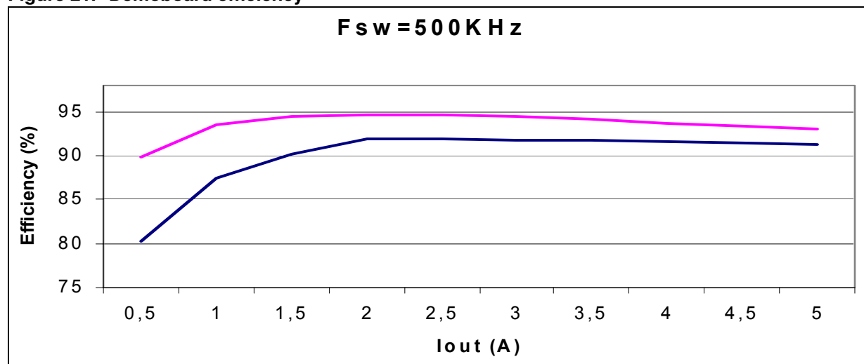
Figure 21. Demoboard efficiency
