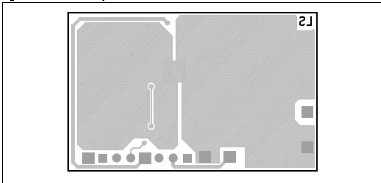
Figure 23. Demoboard layout
