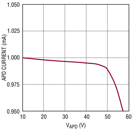
APD Current Regulation vs V_{APD}
