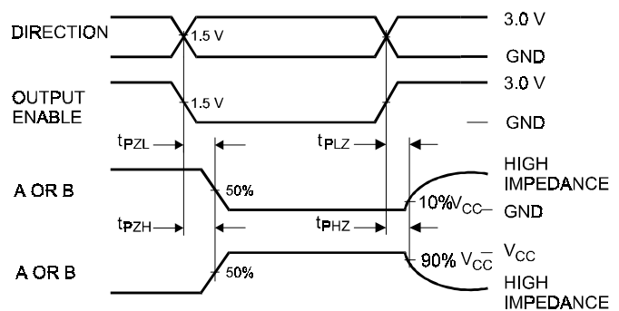
Figure 2. Switching Waveforms
