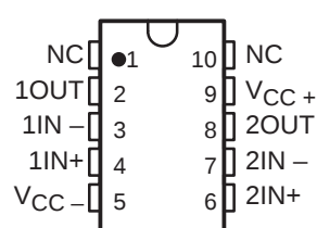
TL288M U PACKAGE (TOP VIEW)
