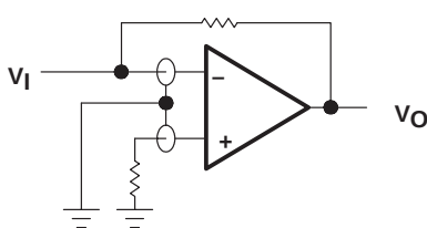
(b) INVERTING AMPLIFIER
