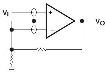
(a) NONINVERTING AMPLIFIER
