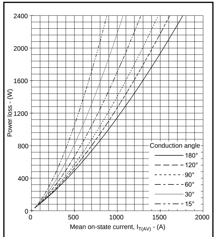
Fig.5 Sine wave power dissipation curves
