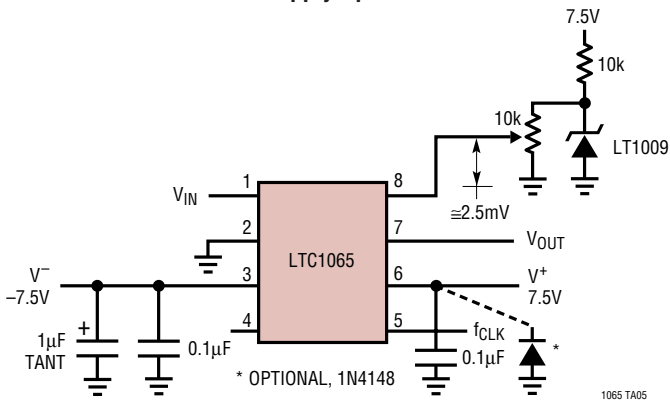
Adjusting V_{OS(OUT)} for \pm 7.5 Supply Operation
