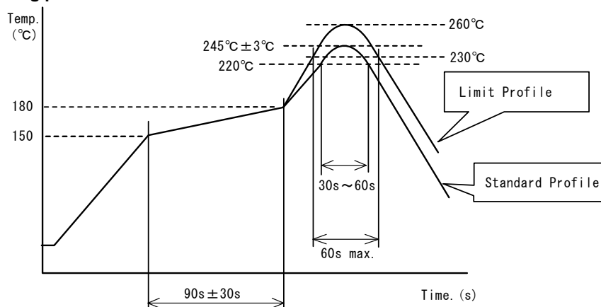
Soldering profile
