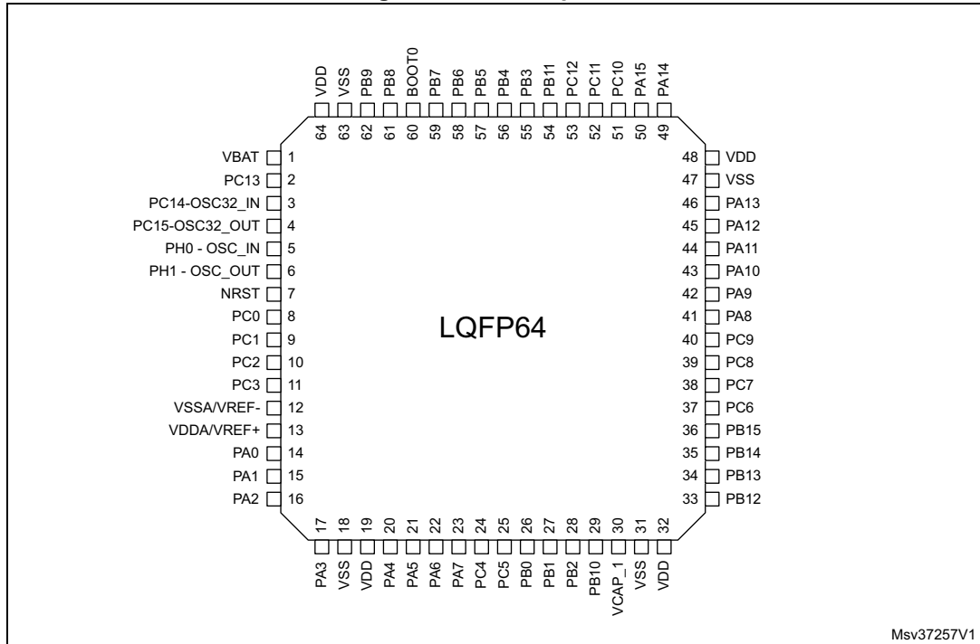
Figure 6. LQFP64 pinout
