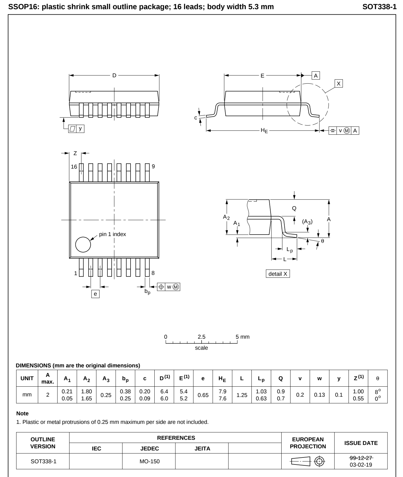
Fig 10. Package outline SOT338-1 (SSOP16)
