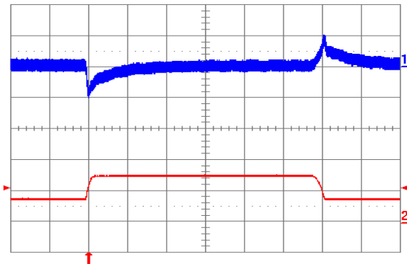
Fig. 3.3V.11: Output voltage response to load current step-change (3.75A – 7.5A – 3.75A) at V_{in} = 24V . Top trace: output voltage (100 mV/div.). Bottom trace: load current (5 A/div.). Current slew rate: 0.1 A/ \mu s . C_o = 1 \mu F ceramic. Time scale: 0.2 ms/div.
