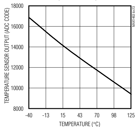
TEMPERATURE SENSOR OUTPUT vs. TEMPERATURE
