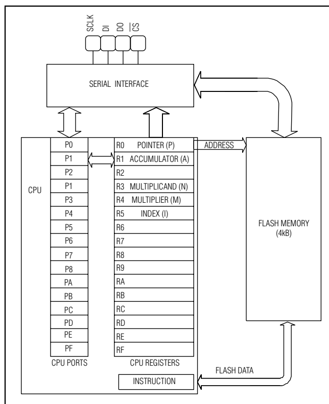
Figure 3. CPU Architecture
