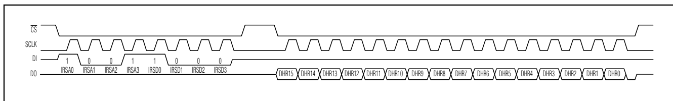
Figure 11. 3-Wire Mode Data Read from DHR Register
