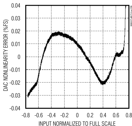
DAC INL
