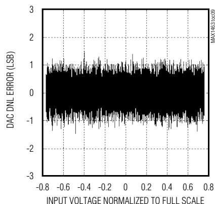
DAC DNL
