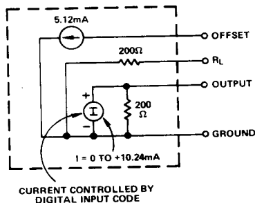
Figure 1. HDS Current Equivalent Circuit
