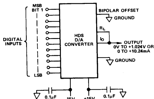
Figure 4. Unipolar Current Output
