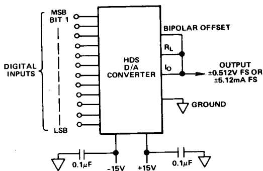
Figure 3. Bipolar Current Output
