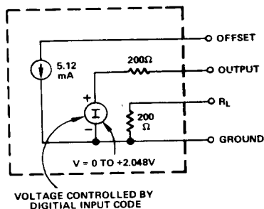
Figure 2. HDS Voltage Equivalent Circuit
