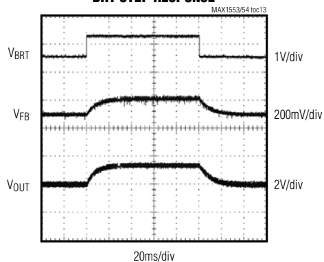
BRT STEP RESPONSE
