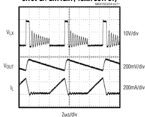
SWITCHING WAVEFORMS (DISCONTINUOUS OPERATION, 3.75V Li+ BATTERY, 10mA OUTPUT)
