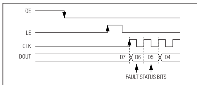
Figure 4. Fault Timing
