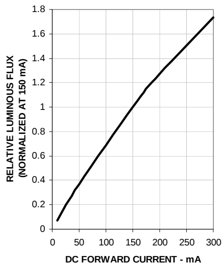
Relative Luminous Flux vs. Forward Current
