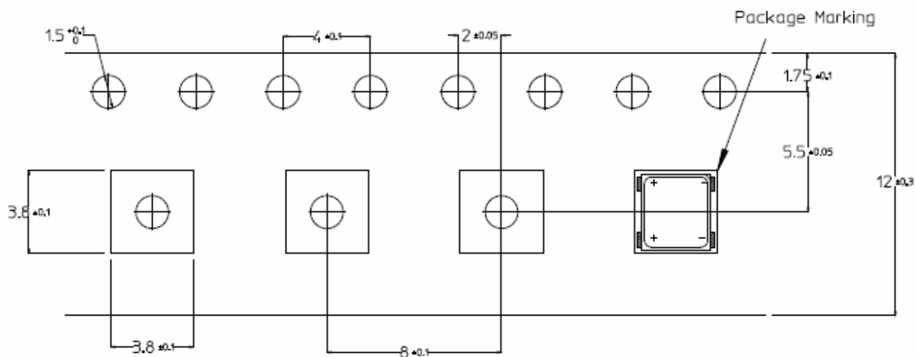
Carrier Tape
