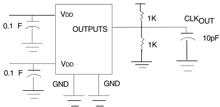
TEST CIRCUIT 2
