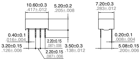
External dimensions
