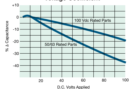
Voltage Coefficient
