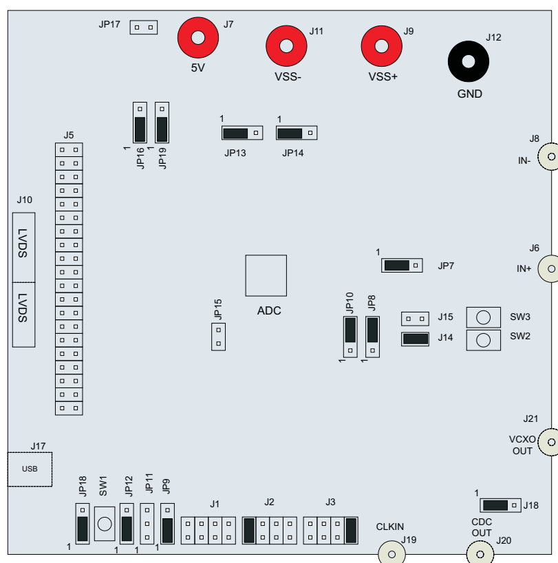
Figure 1. ADS61x9/55xx Jumpers
