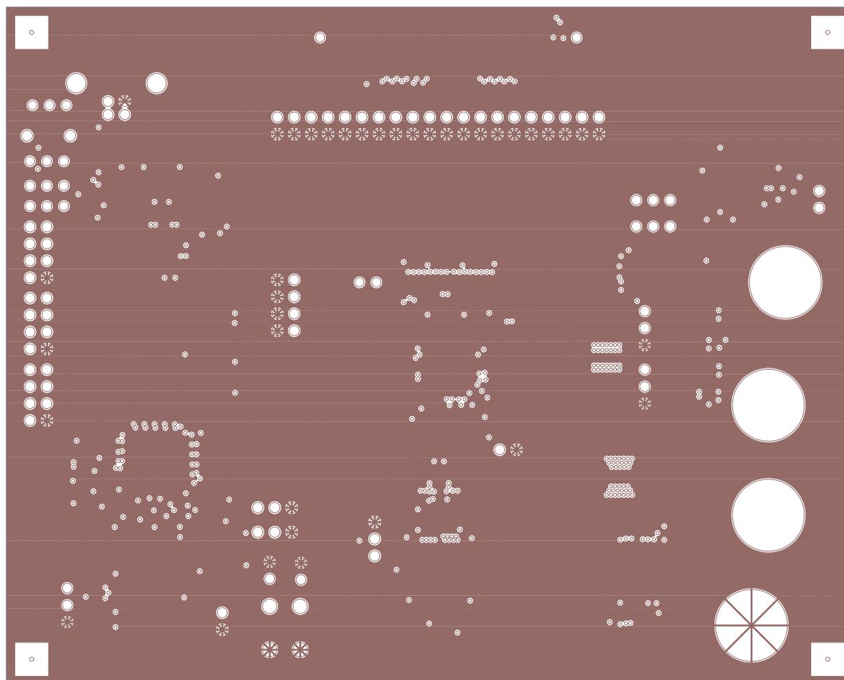
Figure 12. Ground Plane 1
