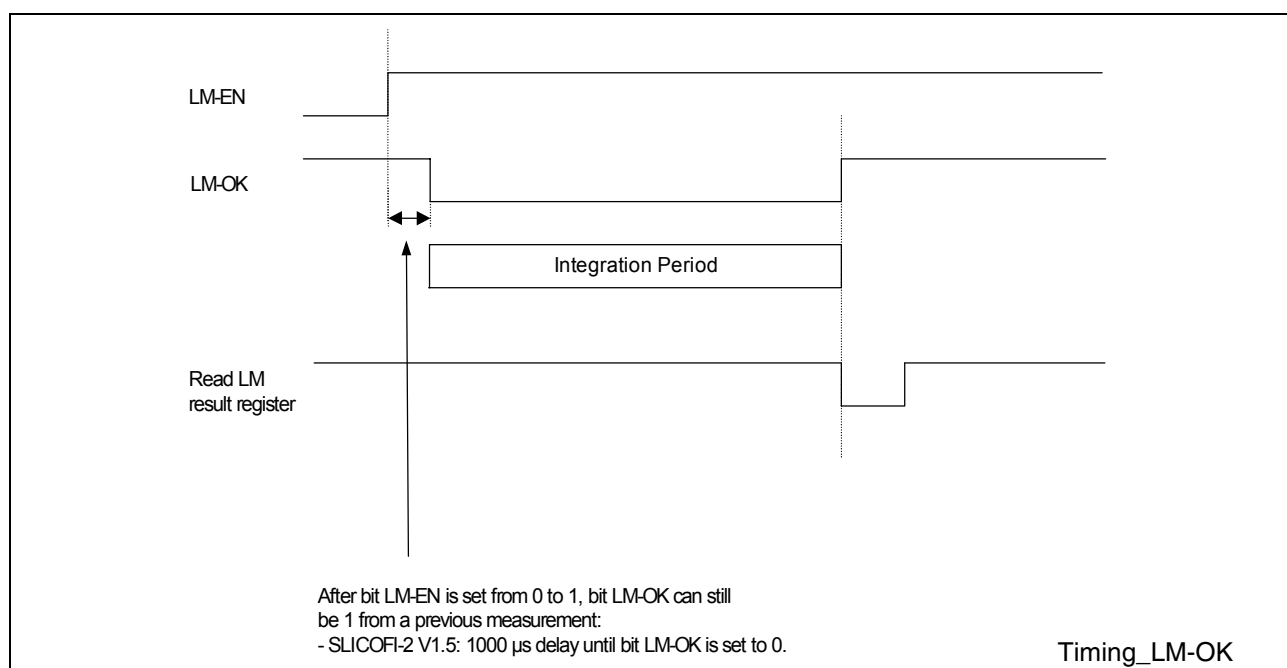
Figure 44 Timing LM-OK Bit
