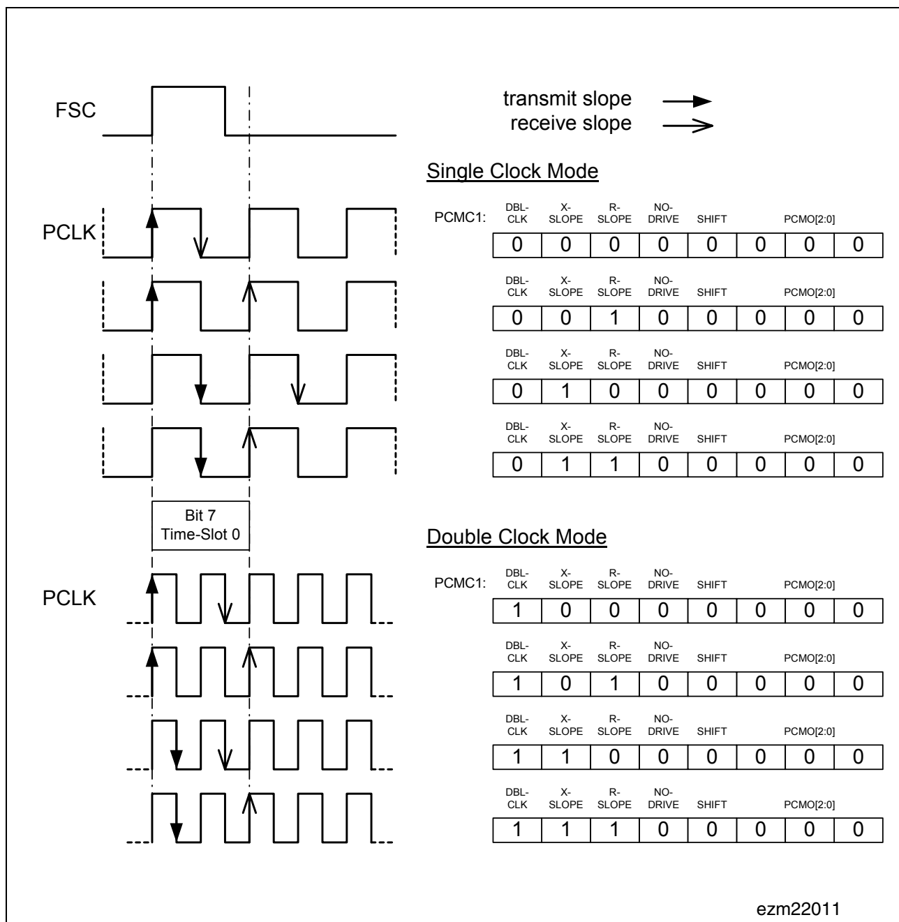
Figure 53 Setting the Slopes in Register PCMC1
