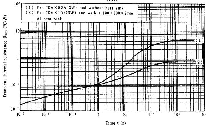
R_{th(t)} - t
