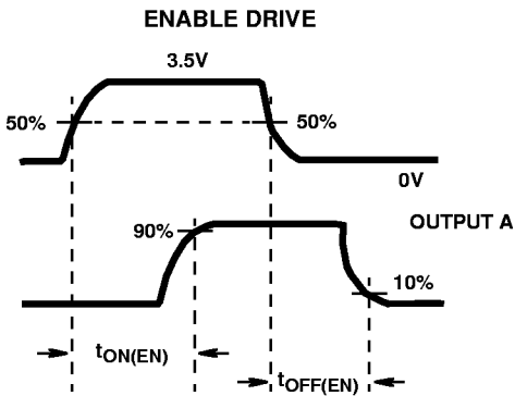
FIGURE 10B. WAVEFORMS
