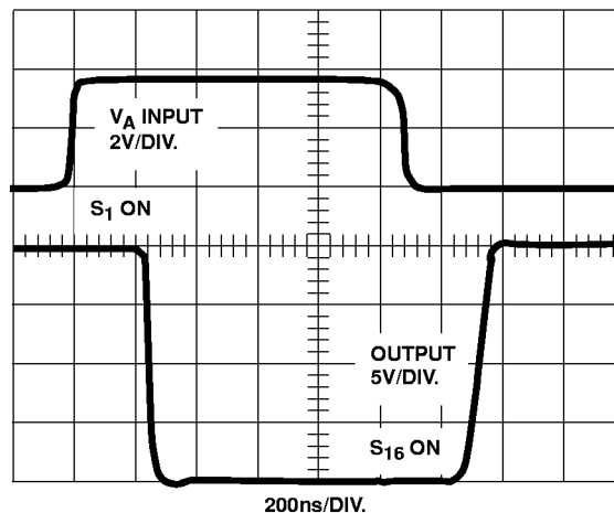
FIGURE 8D. ACCESS TIME
