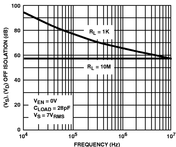
FIGURE 4. OFF ISOLATION vs FREQUENCY
