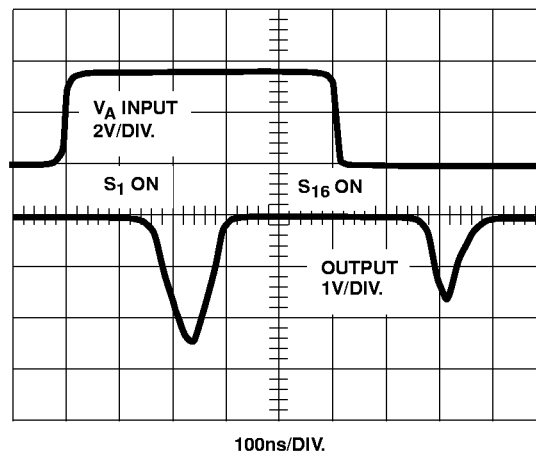
FIGURE 9C. BREAK-BEFORE-MAKE DELAY ( t_{OPEN} )
