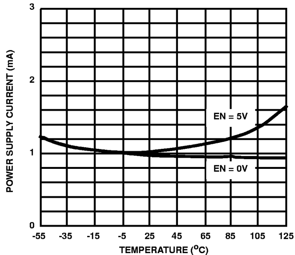
FIGURE 5B. HI-508/HI-509
