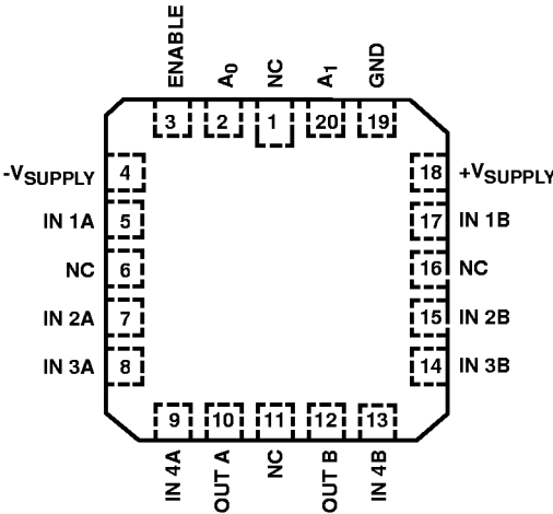
HI-509 (CLCC, PLCC) TOP VIEW
