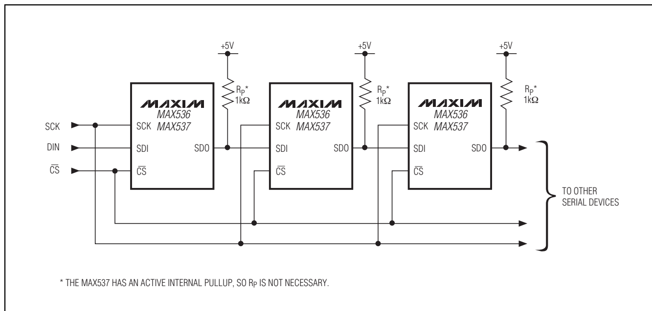
Figure 8. Daisy-Chaining MAX536/MAX537s with a 3-Wire Serial Interface
