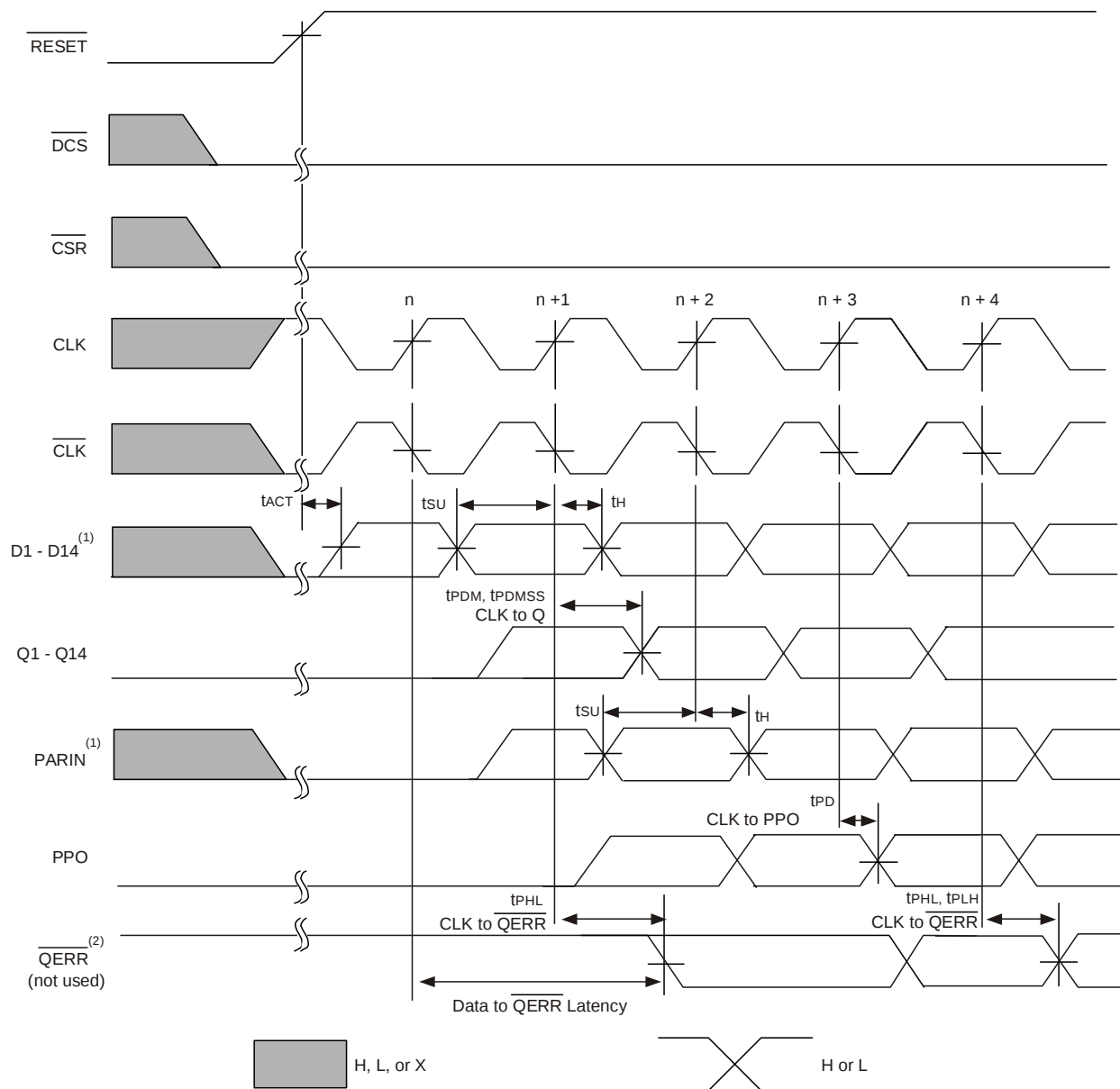
Timing Diagram for the First SSTUBF32866B (1:2 Register-A Configuration) Device Used in a Pair; C0 = 0, C1 = 1, \overline{\text{RESET}} Switches from L to H
