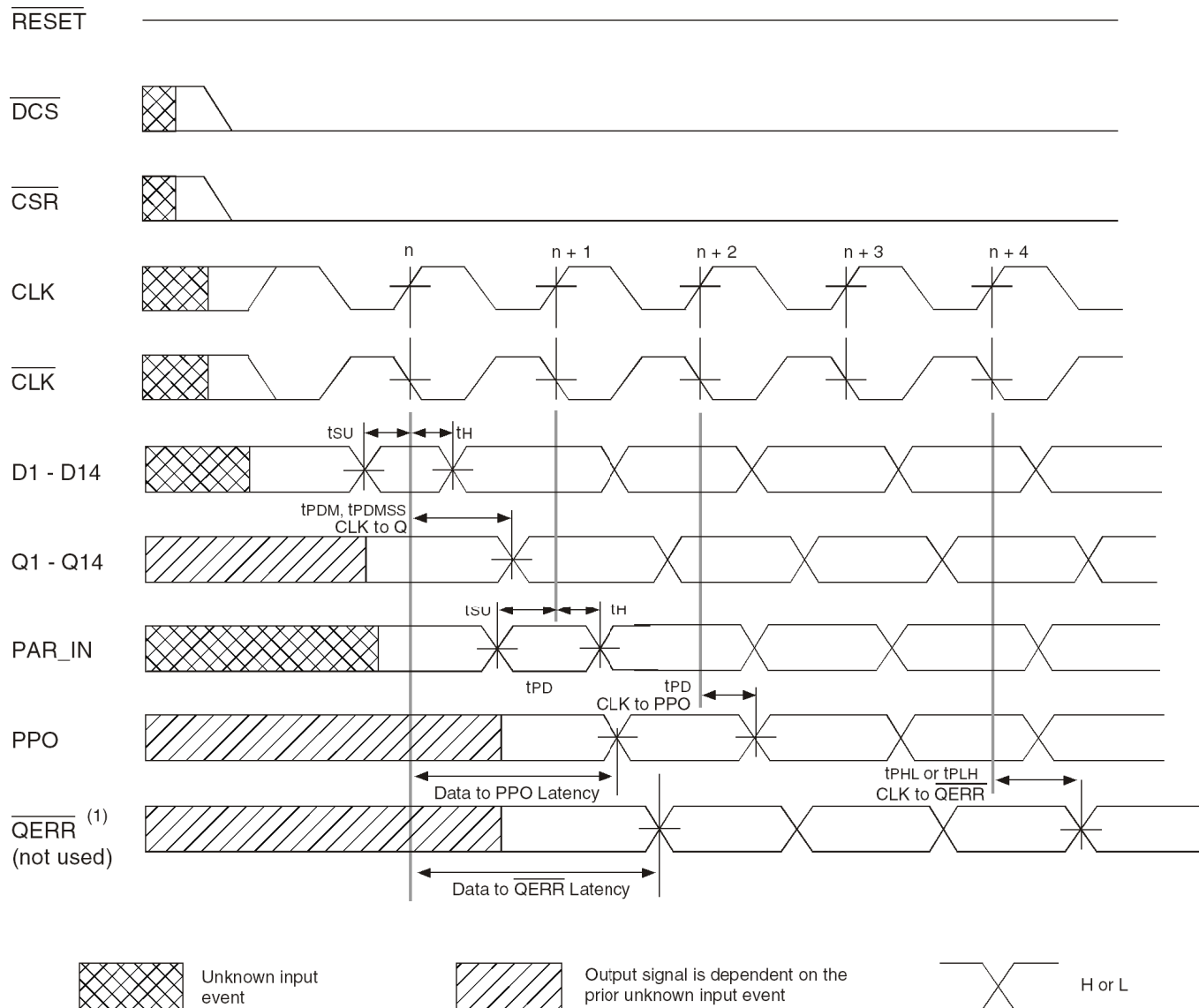
Timing Diagram for the Second SSTUBF32866B (1:2 Register-B Configuration) Device Used in a Pair; C0 = 1, C1 = 1, \overline{\text{RESET}} Held HIGH
