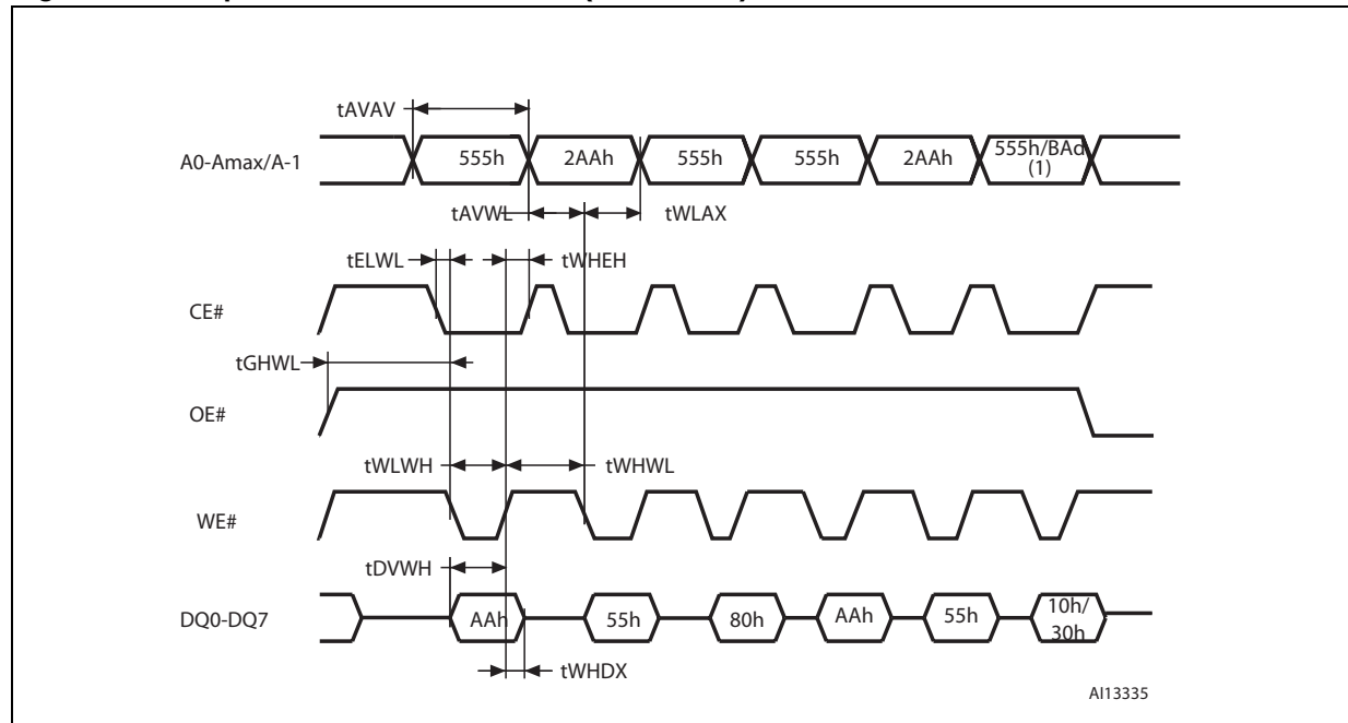
Figure 25. Chip/Block Erase waveforms (8-bit mode)
