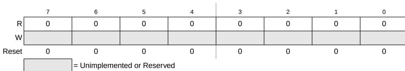
Figure 26-5. RESERVED1
