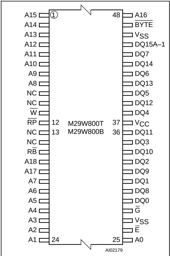
Figure 3. TSOP Connections
