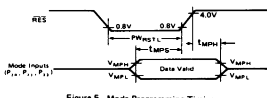
Figure 5 Mode Programming Timing
