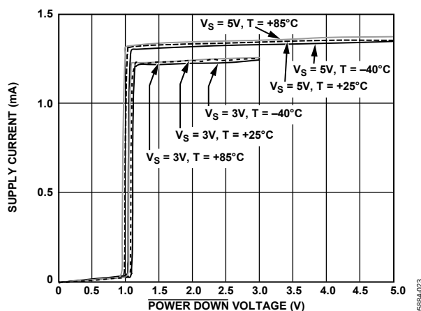
Figure 38. Supply Current vs. \overline{\text{POWER DOWN}} Voltage
