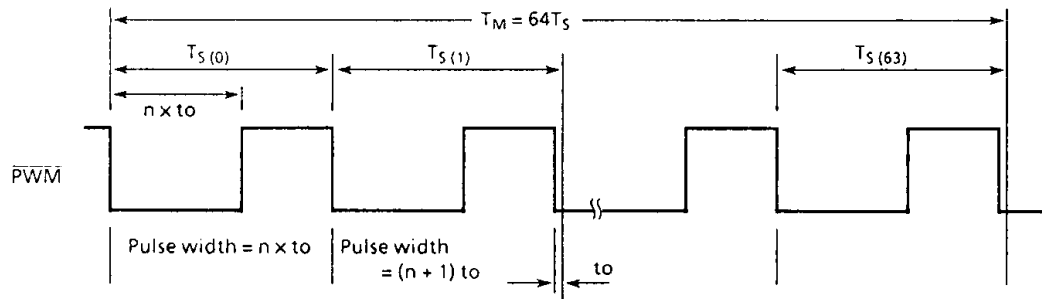
Figure 2-18. \overline{\text{PWM}} output timing (It is shown to the additional pulse T_S(1) and T_S(63) )
