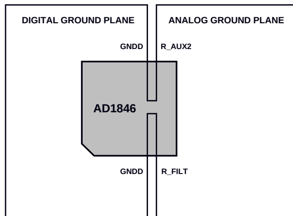
Figure 25. Recommended Ground Plane
