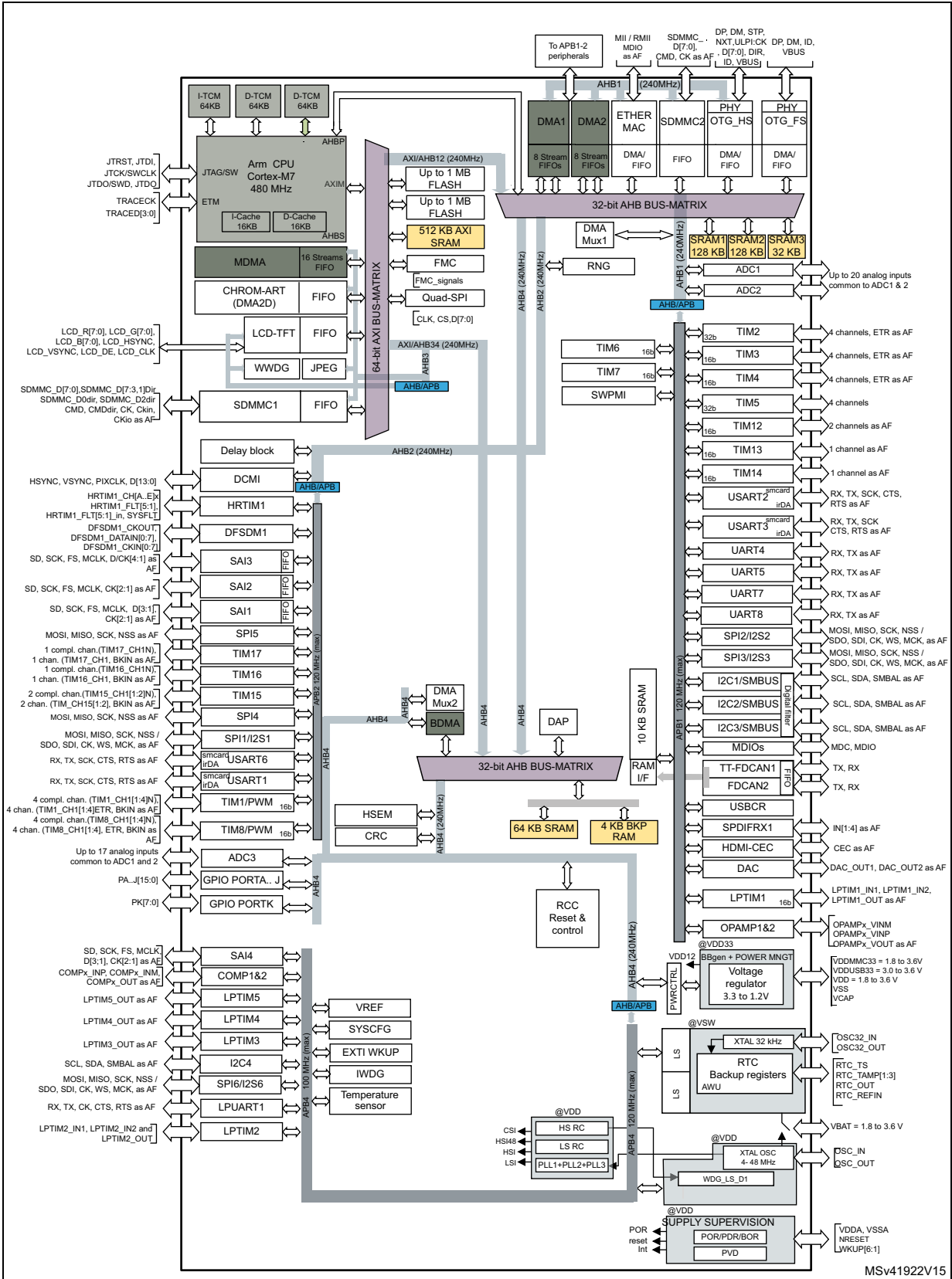
Figure 2. STM32H743xl/G block diagram
