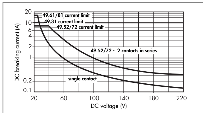
H 49 - Maximum DC1 breaking capacity Types 49.31/52/61/72/81
