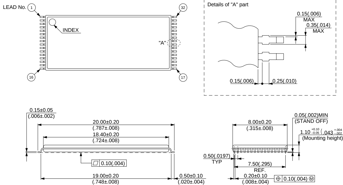
32-pin plastic TSOP(I) (FPT-32P-M24)
