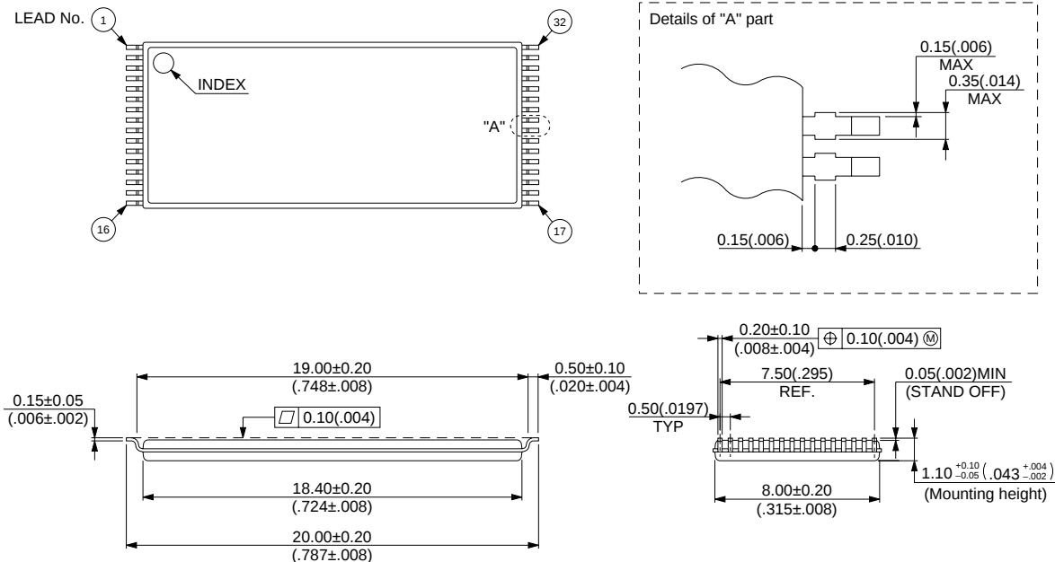
32-pin plastic TSOP(I) (FPT-32P-M25)
