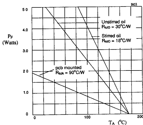
Fig 2. Power derating in air and oil.
