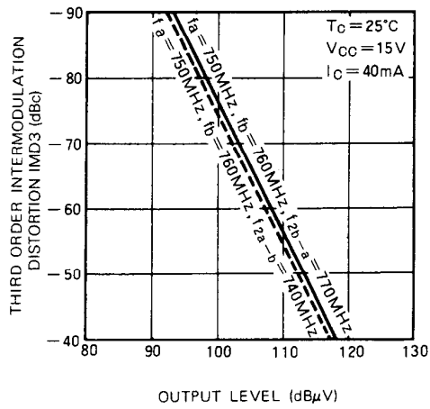
THIRD ORDER INTERMODULATION DISTORTION VS. OUTPUT LEVEL
