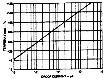
Figure 7. Droop Current vs. Temperature
