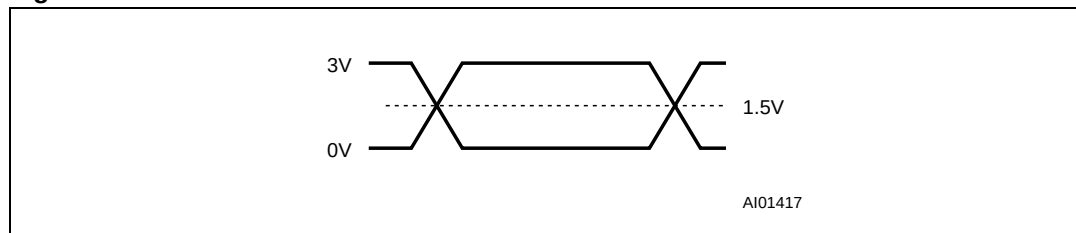
Figure 11. A/A Mux interface AC measurement I/O waveform
