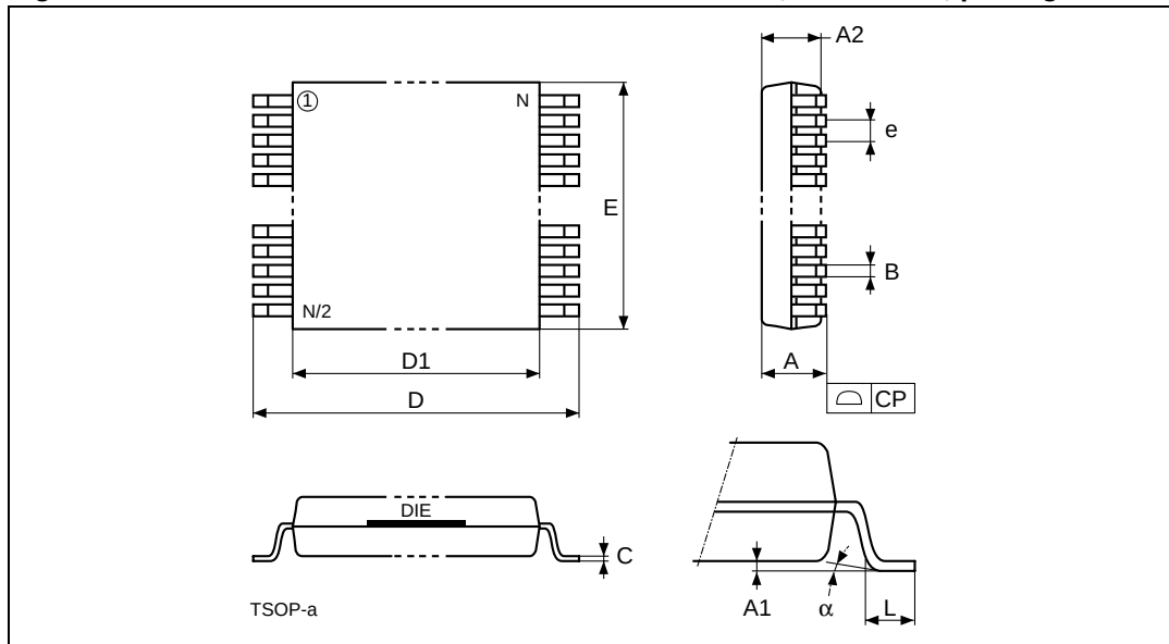
Figure 20. TSOP40 – 40 lead Plastic Thin Small Outline, 10 x 20mm, package outline
