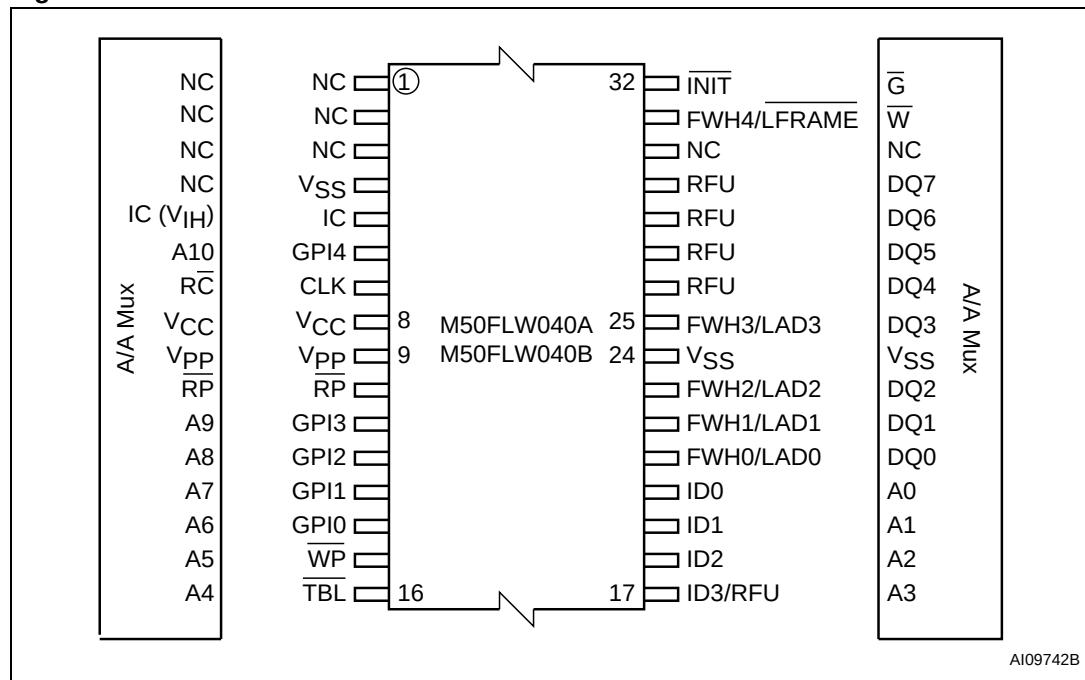
Figure 4. TSOP32 connections
