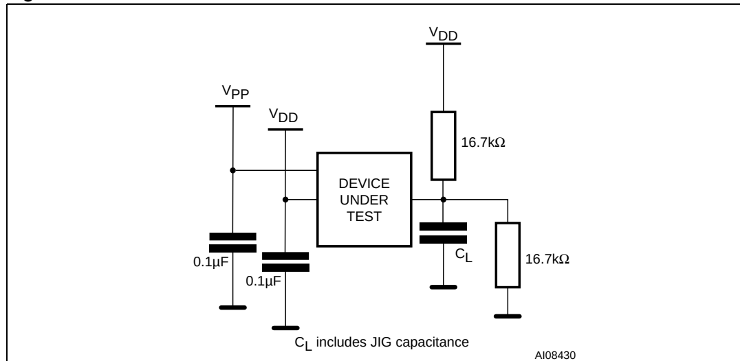
Figure 12. AC measurement load circuit
