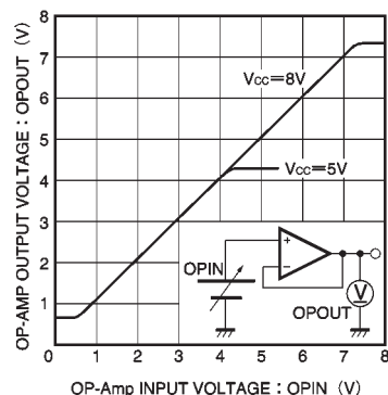
Fig.9 Op-amp I/O characteristics
