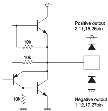
Driver output
