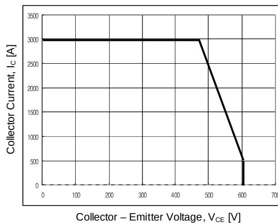
Fig 10. SCSOA characteristics
