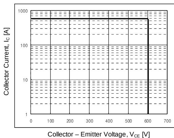
Fig 9. RBSOA characteristics
