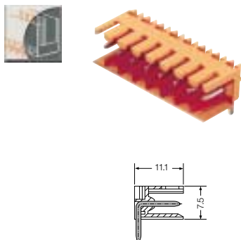
Pin headers SL 3.5/90
