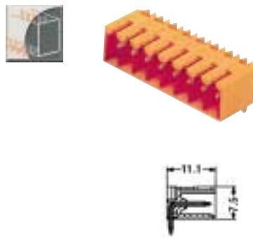
Pin headers SL 3.5/90G
