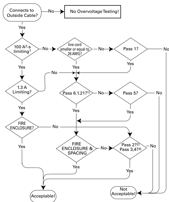
Figure 3.19 Overvoltage Flowchart
