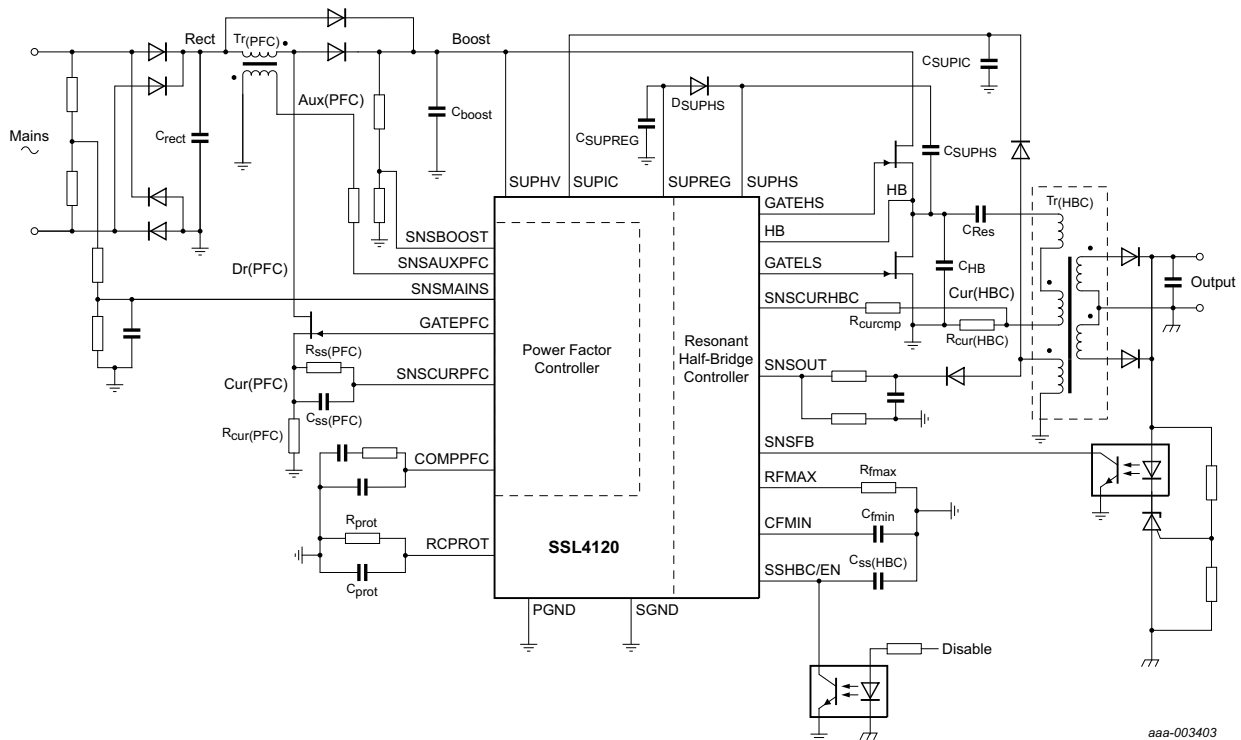
Fig 19. Application diagram of SSL4120T
