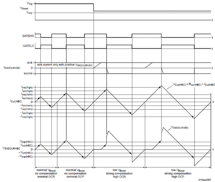
Fig 17. Boost voltage compensation
