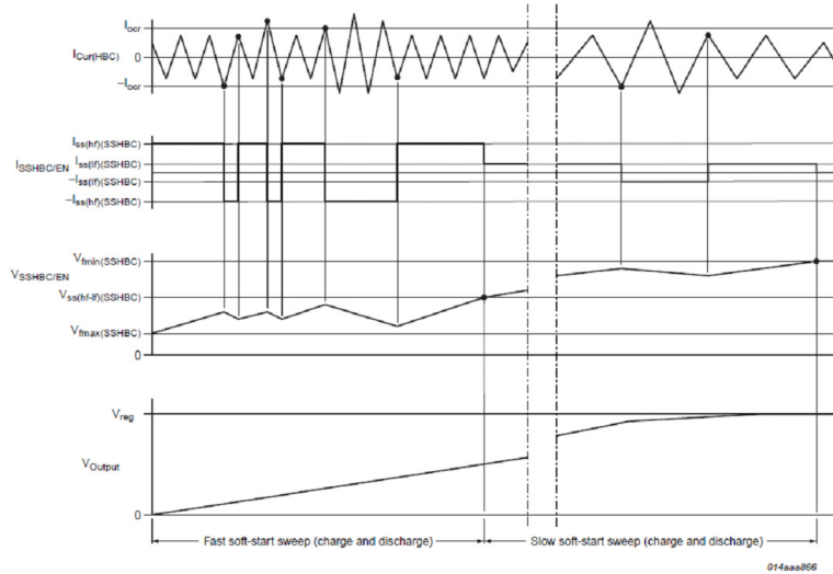
Fig 18. Overcurrent regulation during start-up
