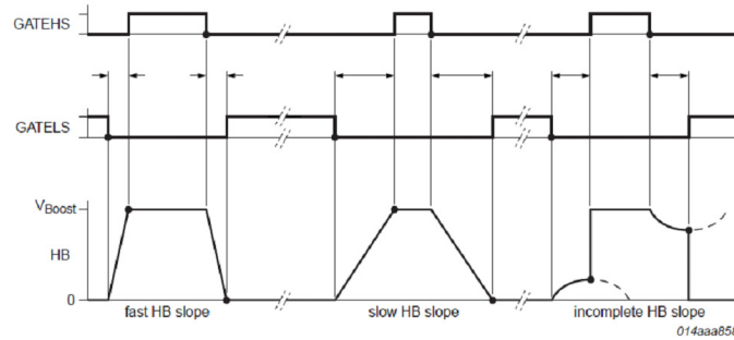
Fig 10. Adaptive non-overlap time function (normal inductive operation)
