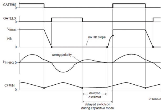
Fig 11. Adaptive non-overlap time function (capacitive operation)
