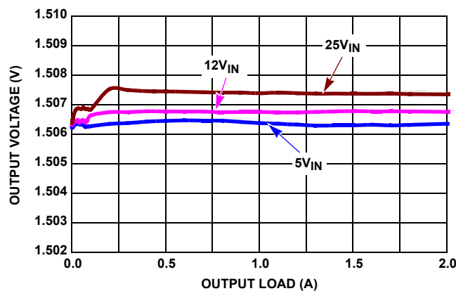
FIGURE 7. V OUT REGULATION vs LOAD, 1.5V OUT
