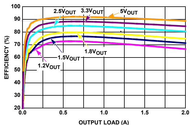
FIGURE 3. EFFICIENCY vs LOAD, 12V IN
