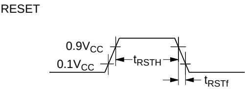
Figure 106 Reset Timing
