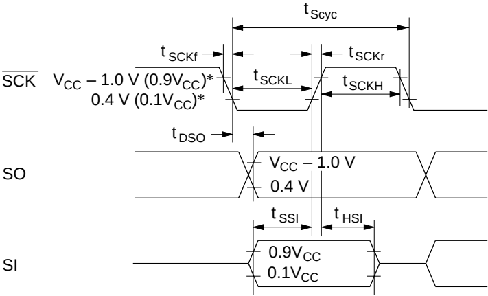
Figure 107 \overline{\text{STOPC}} Timing
