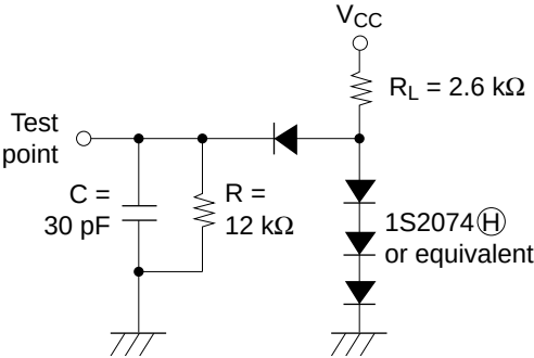
Figure 109 Timing Load Circuit
