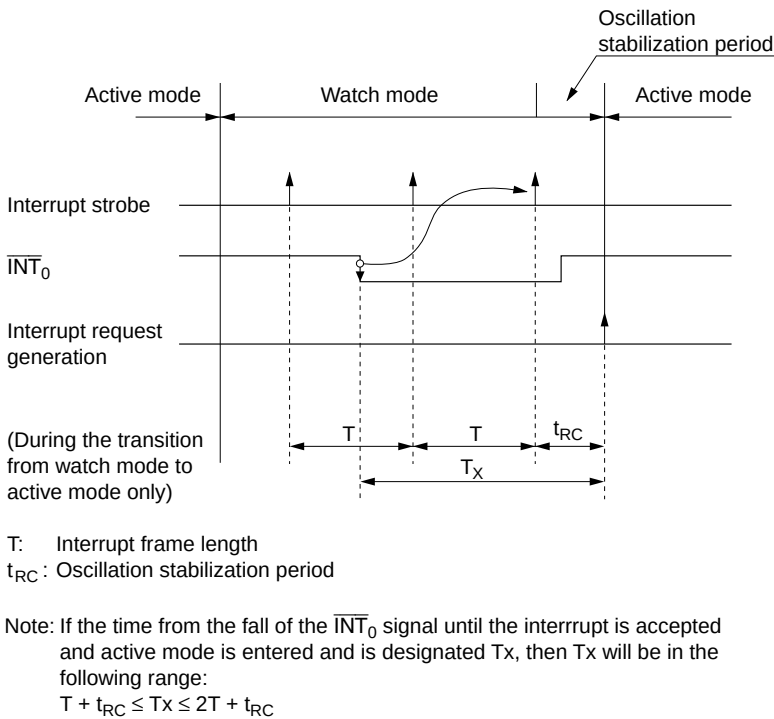
Figure 17 Interrupt Frame
