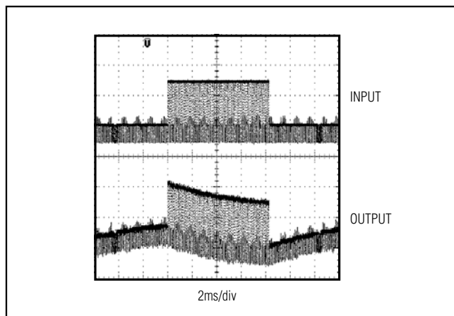
Figure 1. AC-Coupled Output
