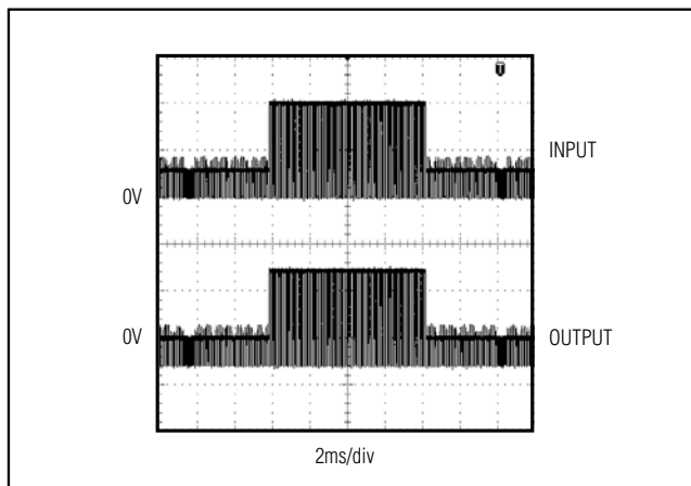
Figure 2. DirectDrive Output
