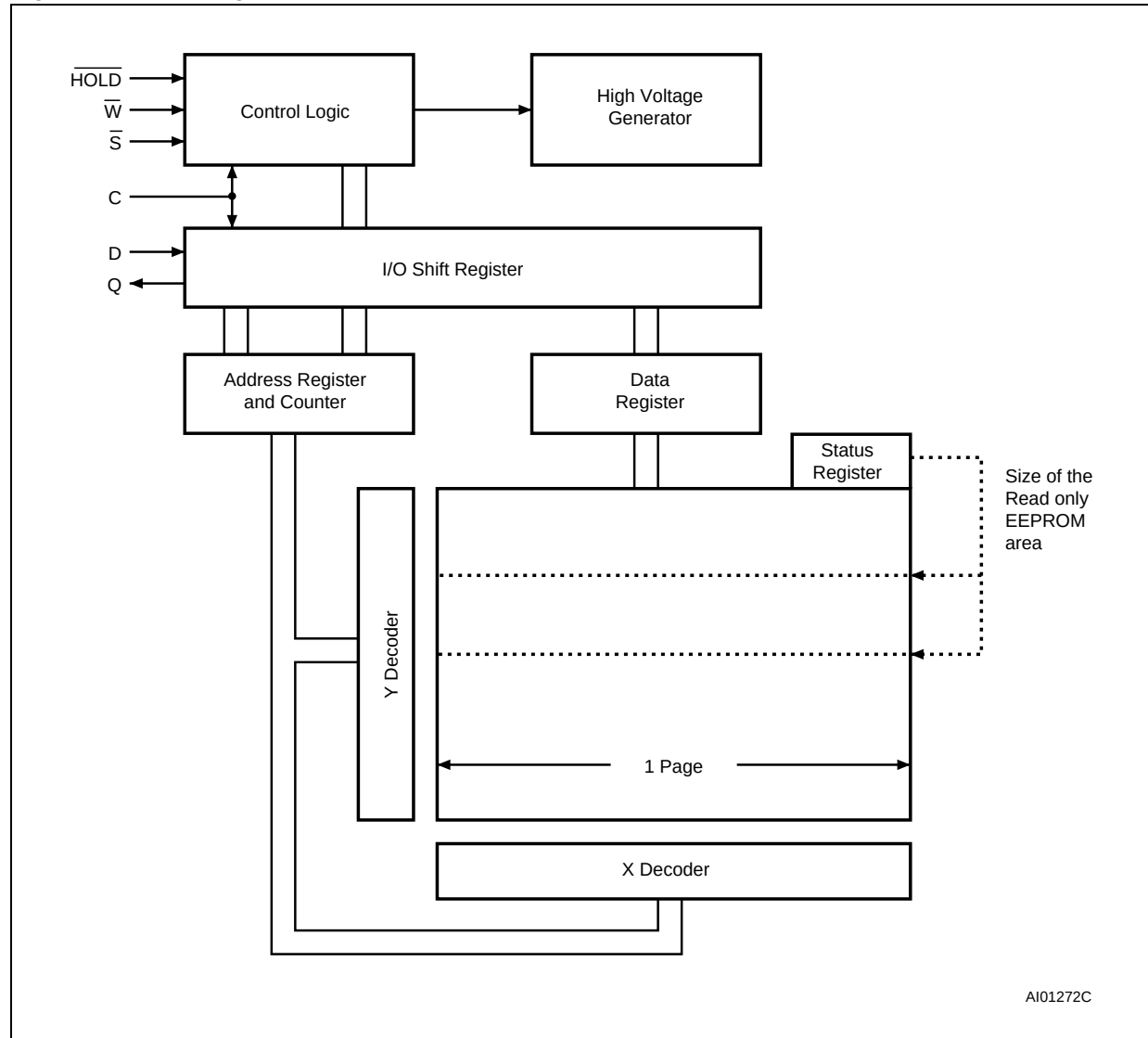
Figure 7. Block Diagram
