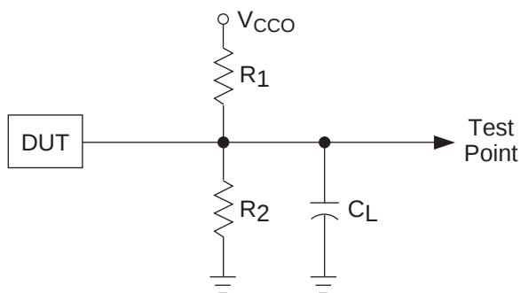
Figure 11. Output Test Load, LVTTTL and LVC MOS Standards
