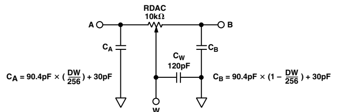
Figure 8. RDAC Circuit Simulation Model for RDAC = 10 kΩ
