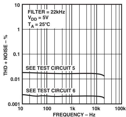
TPC 16. Total Harmonic Distortion Plus Noise vs. Frequency
