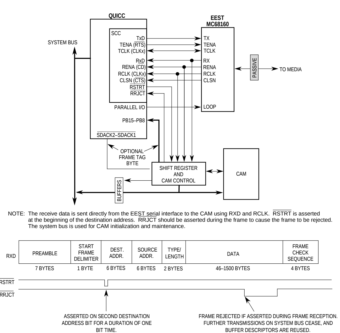
Figure 7-68. QUICC Ethernet Serial CAM Interface
