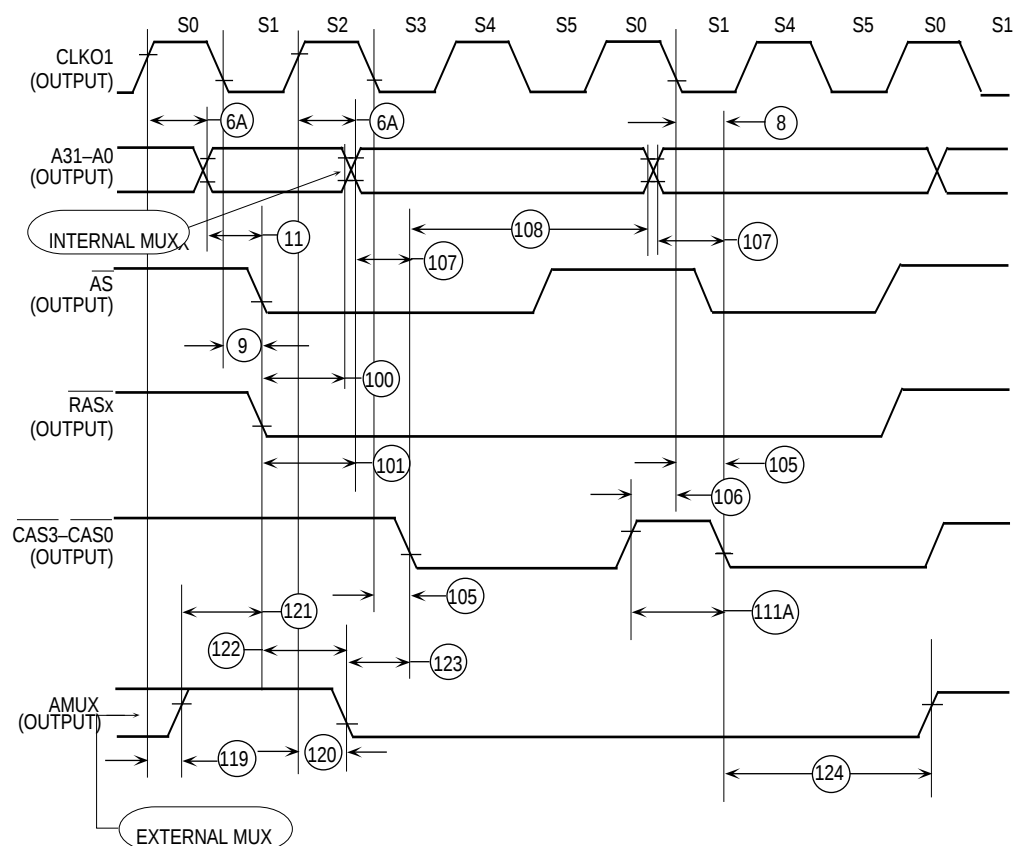
Figure 10-23. DRAM: Page-Mode—Page-Hit
