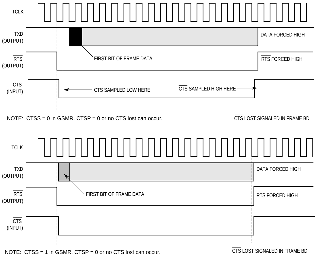
Figure 7-41. CTS Lost in Synchronous Protocols
