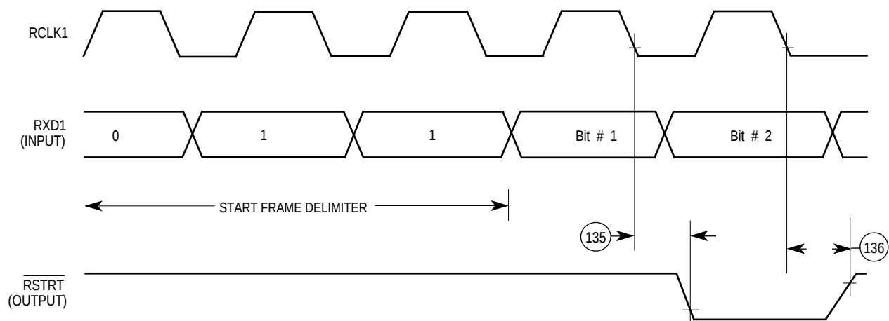
Figure 10-71. CAM Interface Receive Start Timing
