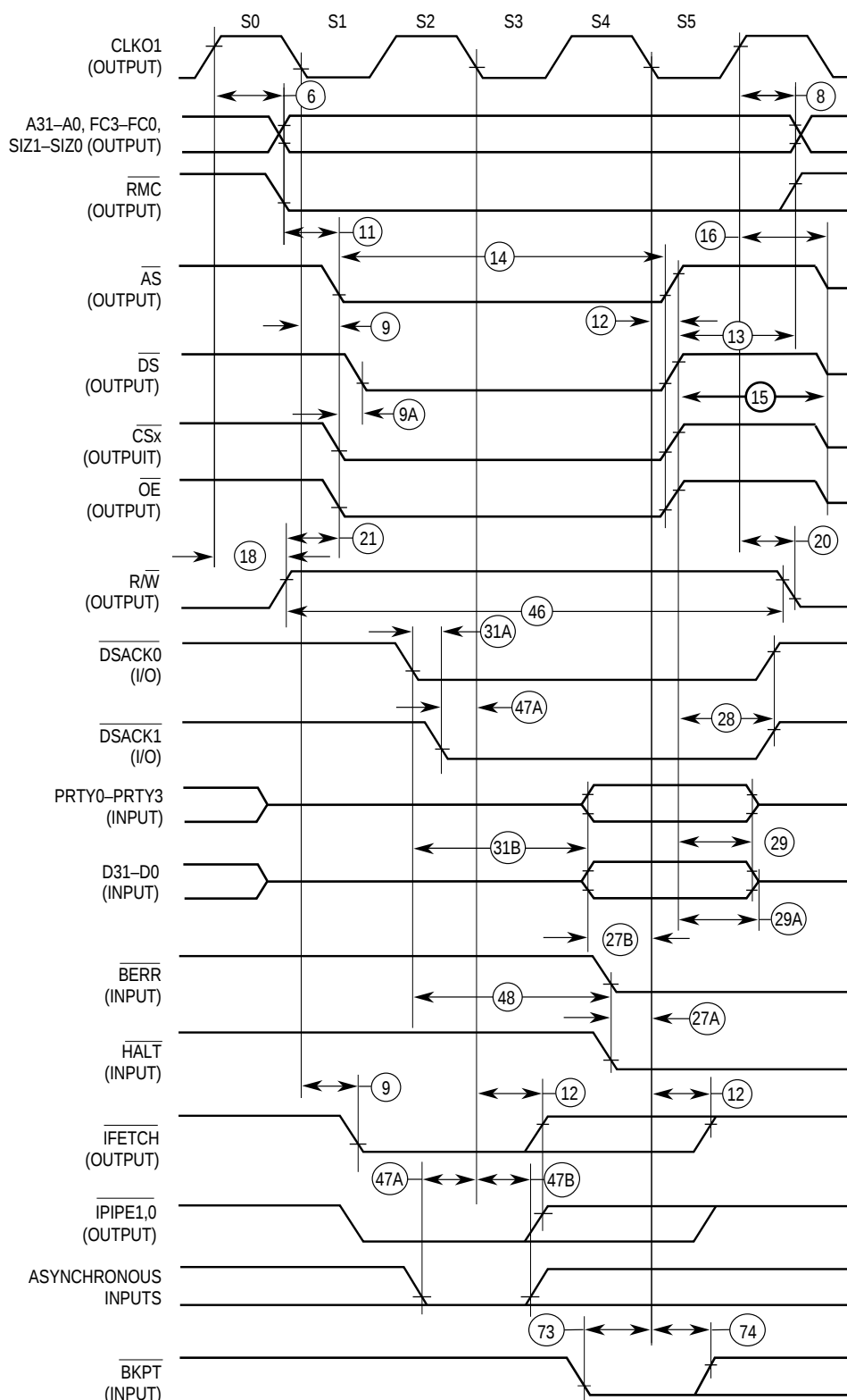
Figure 10-5. Read Cycle (With Parity Check, PBEE = 1)
